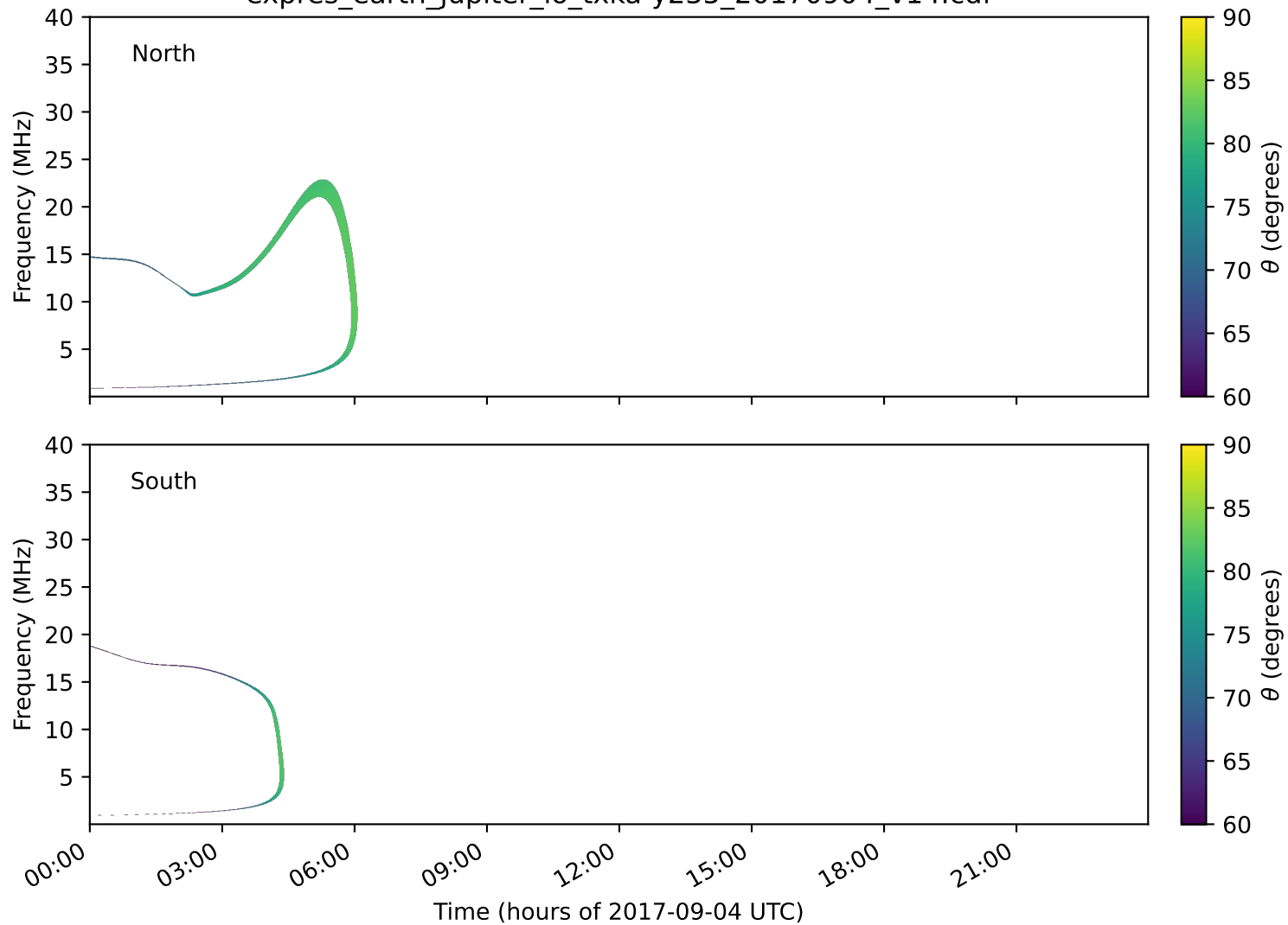
expres_earth_jupiter_io_txka-y235_20170904_v14.cdf
