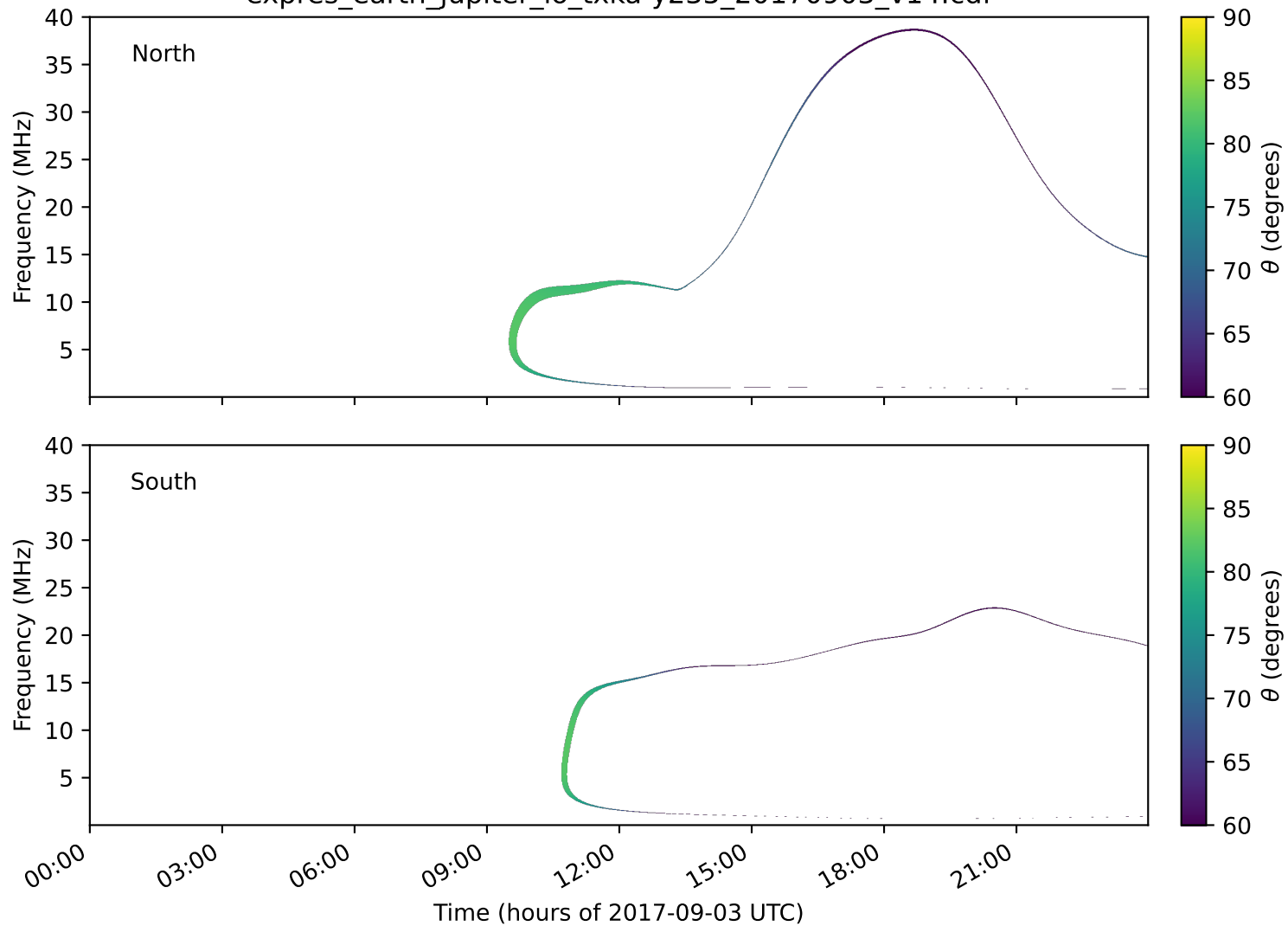
expres_earth_jupiter_io_txka-y235_20170903_v14.cdf
