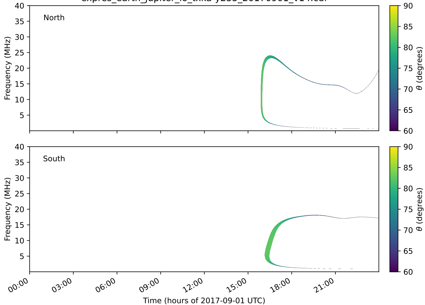
expres_earth_jupiter_io_txka-y235_20170901_v14.cdf
