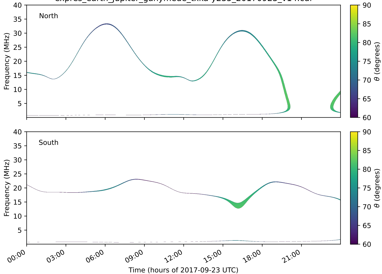
expres_earth_jupiter_ganymede_txka-y235_20170923_v14.cdf
