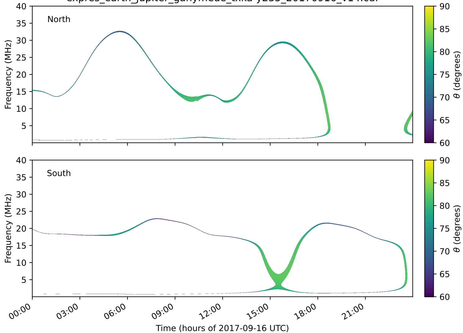
expres_earth_jupiter_ganymede_txka-y235_20170916_v14.cdf
