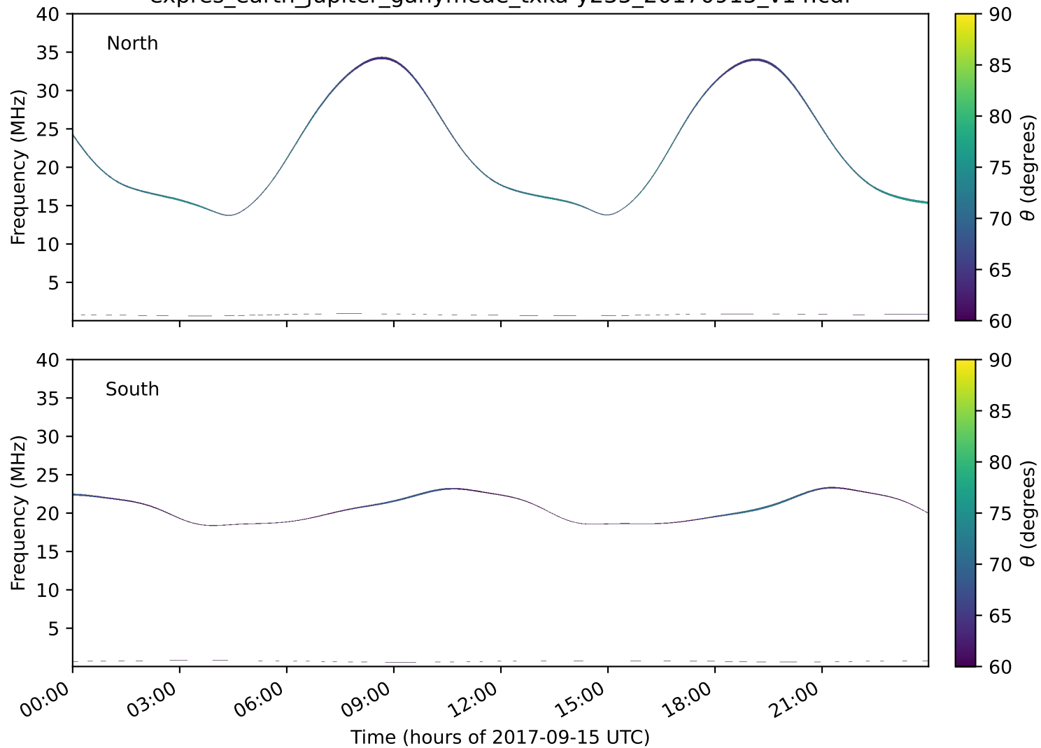
expres_earth_jupiter_ganymede_txka-y235_20170915_v14.cdf
