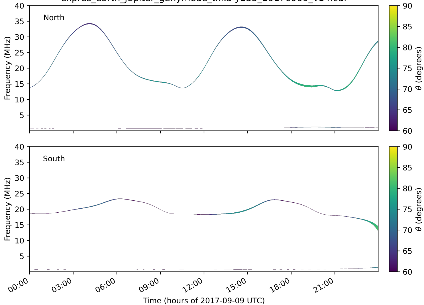
expres_earth_jupiter_ganymede_txka-y235_20170909_v14.cdf
