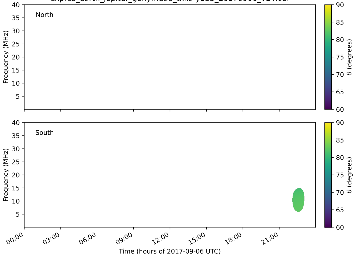
expres_earth_jupiter_ganymede_txka-y235_20170906_v14.cdf
