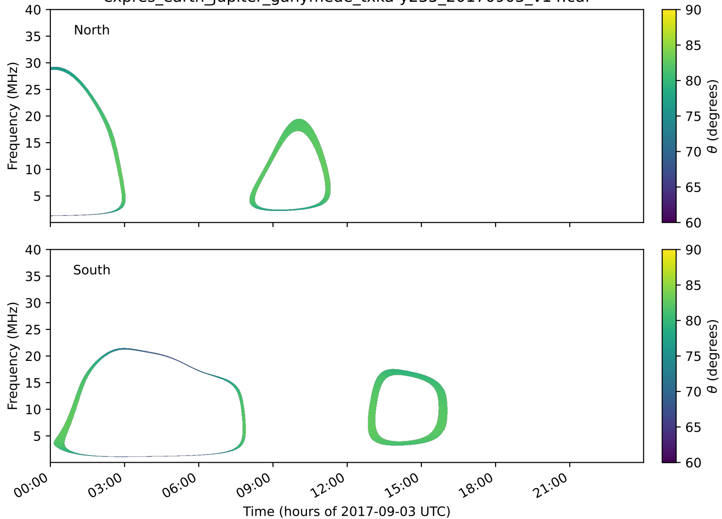
expres_earth_jupiter_ganymede_txka-y235_20170903_v14.cdf
