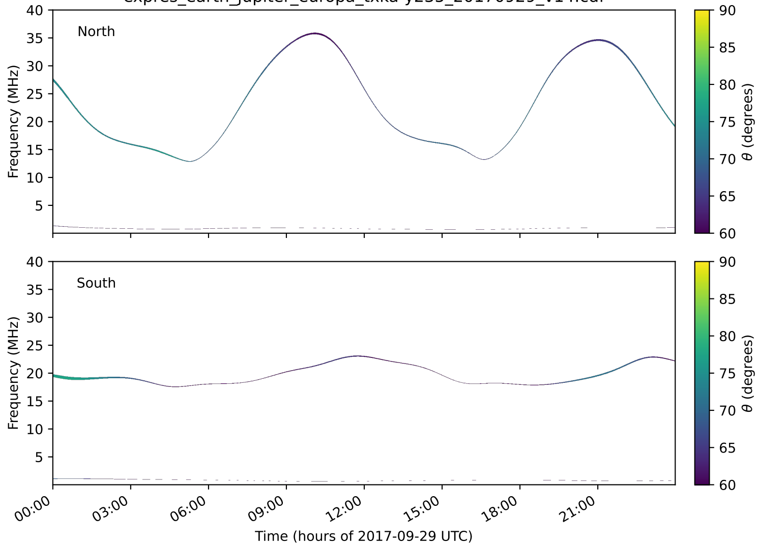
expres_earth_jupiter_europa_txka-y235_20170929_v14.cdf
