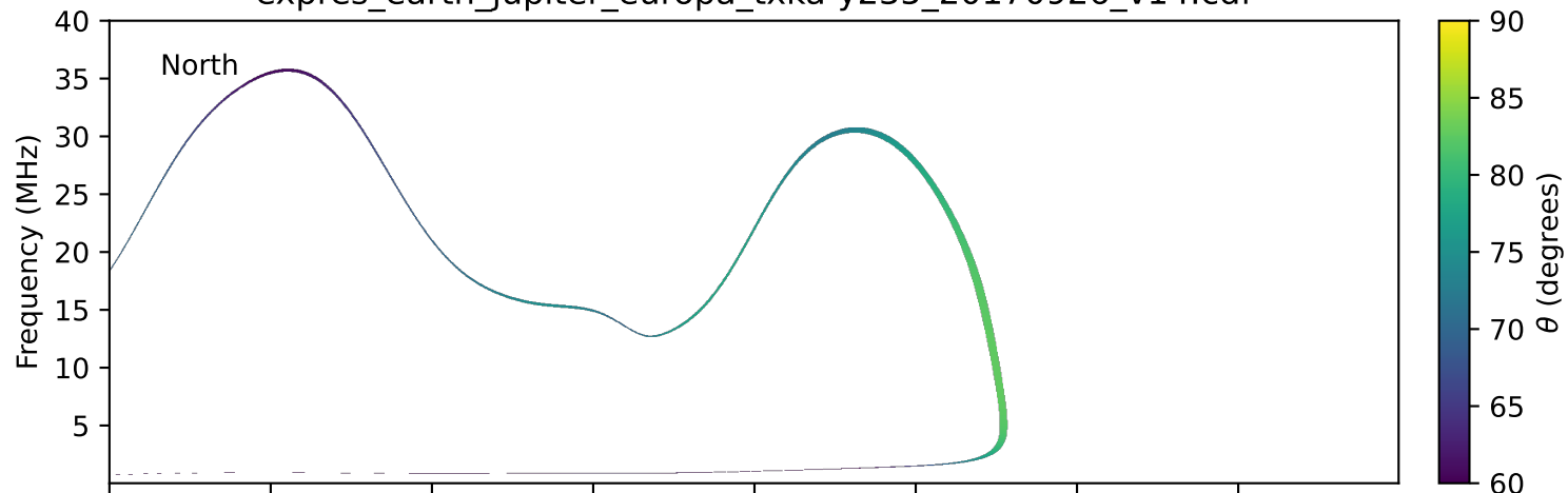
expres_earth_jupiter_europa_txka-y235_20170926_v14.cdf
