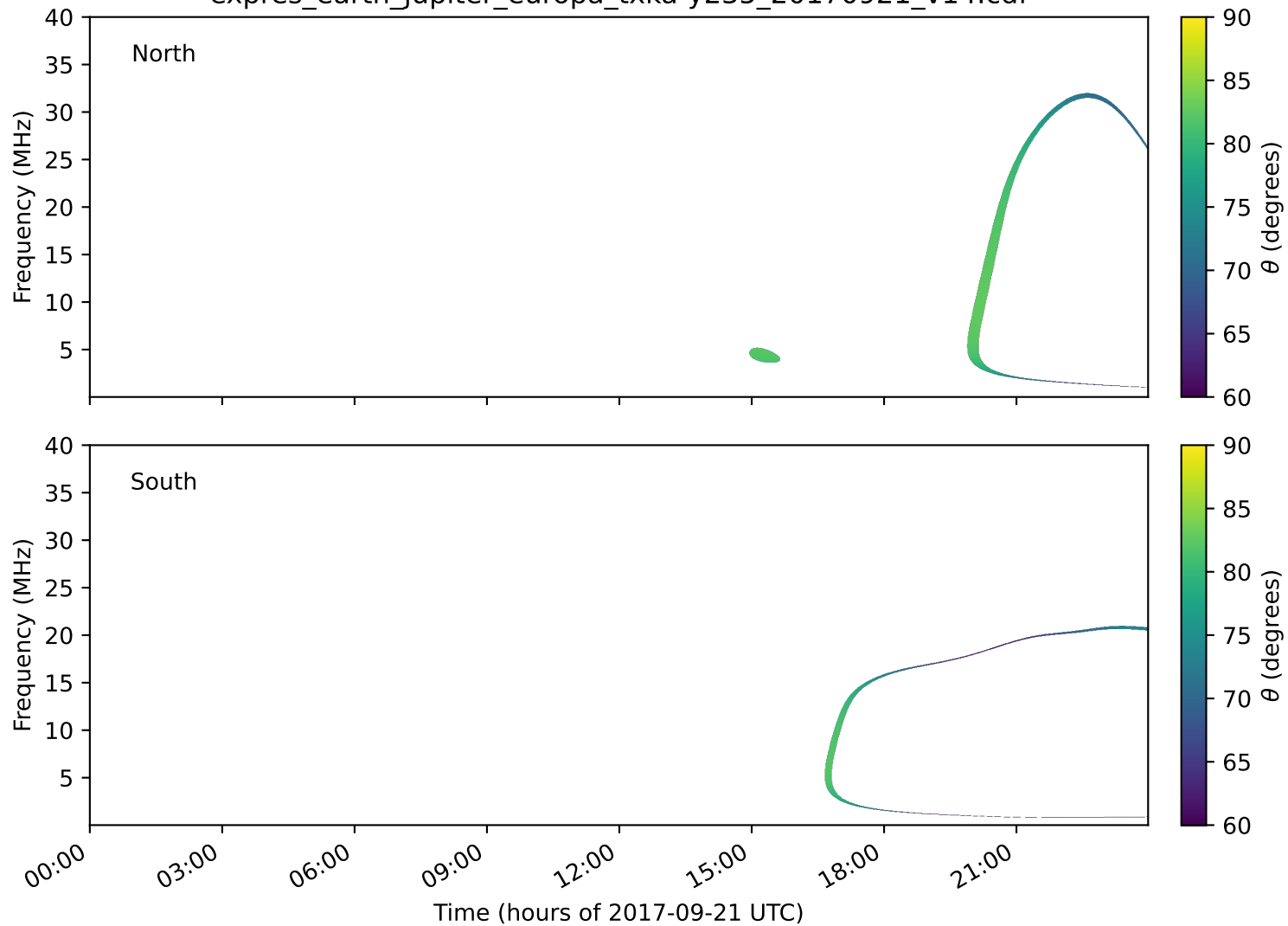
expres_earth_jupiter_europa_txka-y235_20170921_v14.cdf
