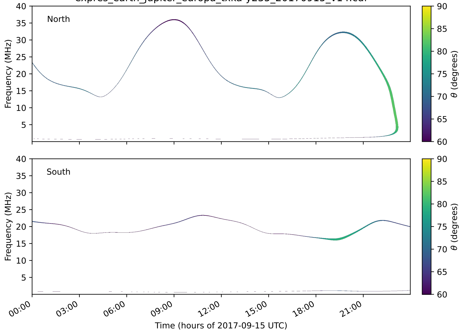
expres_earth_jupiter_europa_txka-y235_20170915_v14.cdf
