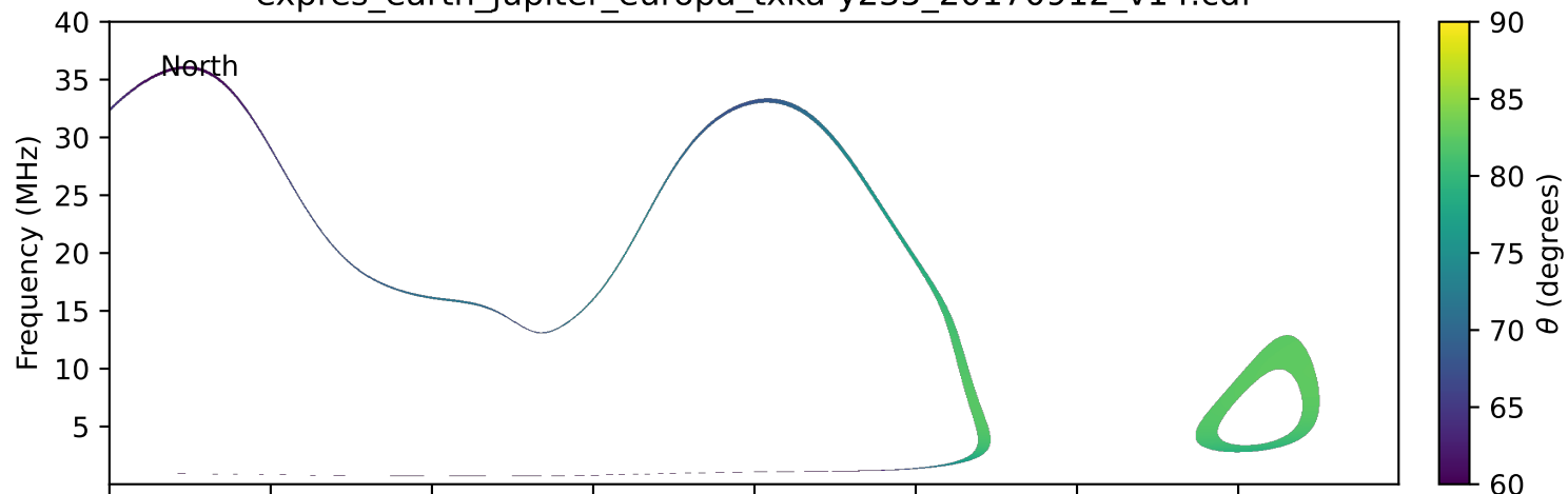
expres_earth_jupiter_europa_txka-y235_20170912_v14.cdf
