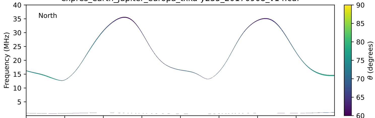
expres_earth_jupiter_europa_txka-y235_20170908_v14.cdf
