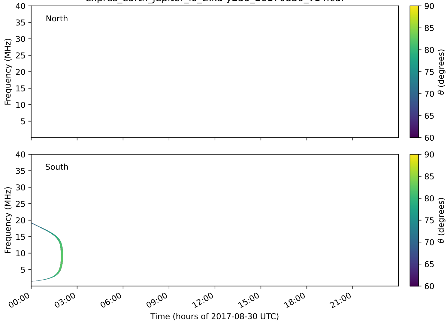
expres_earth_jupiter_io_txka-y235_20170830_v14.cdf
