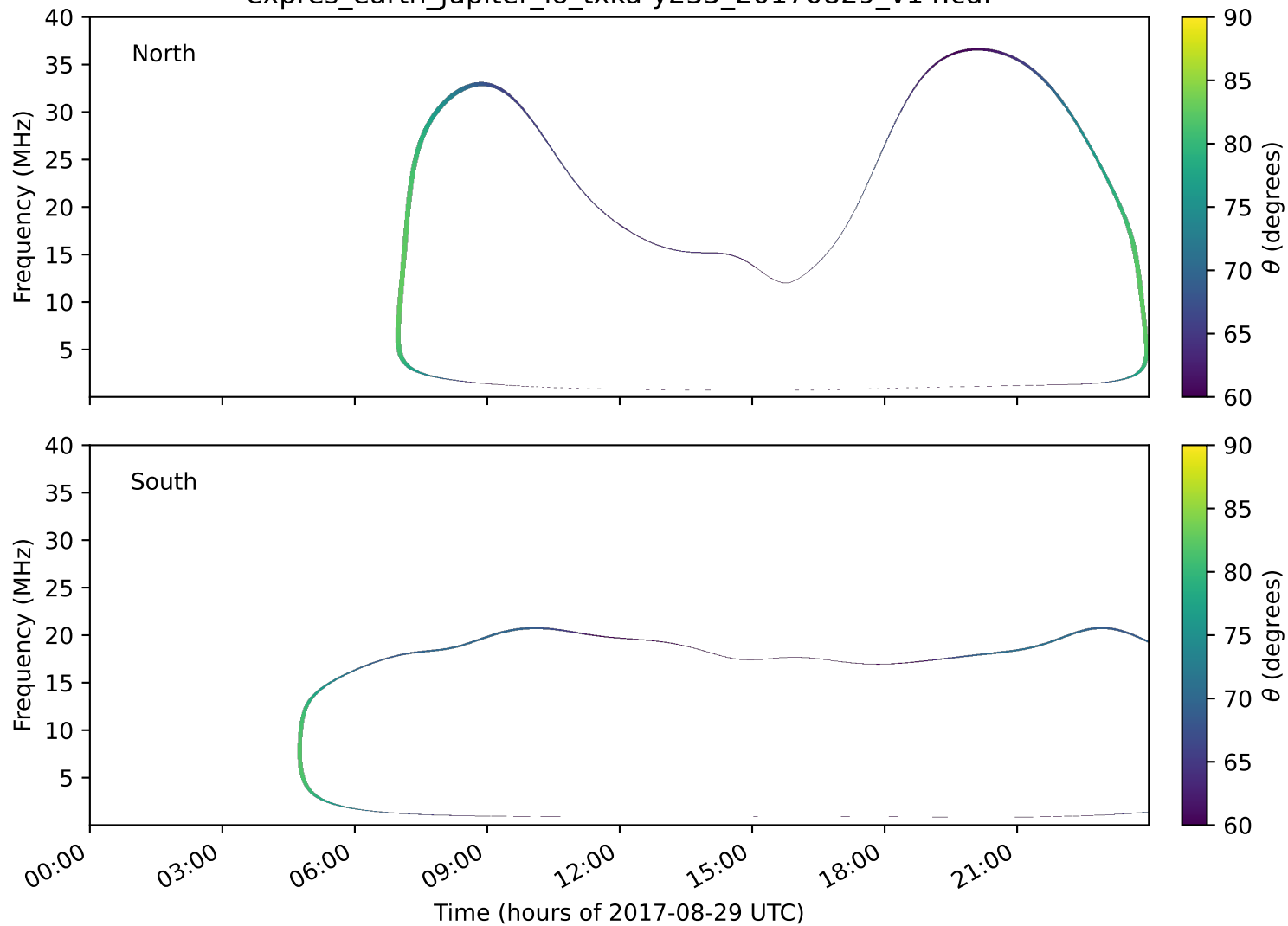
expres_earth_jupiter_io_txka-y235_20170829_v14.cdf
