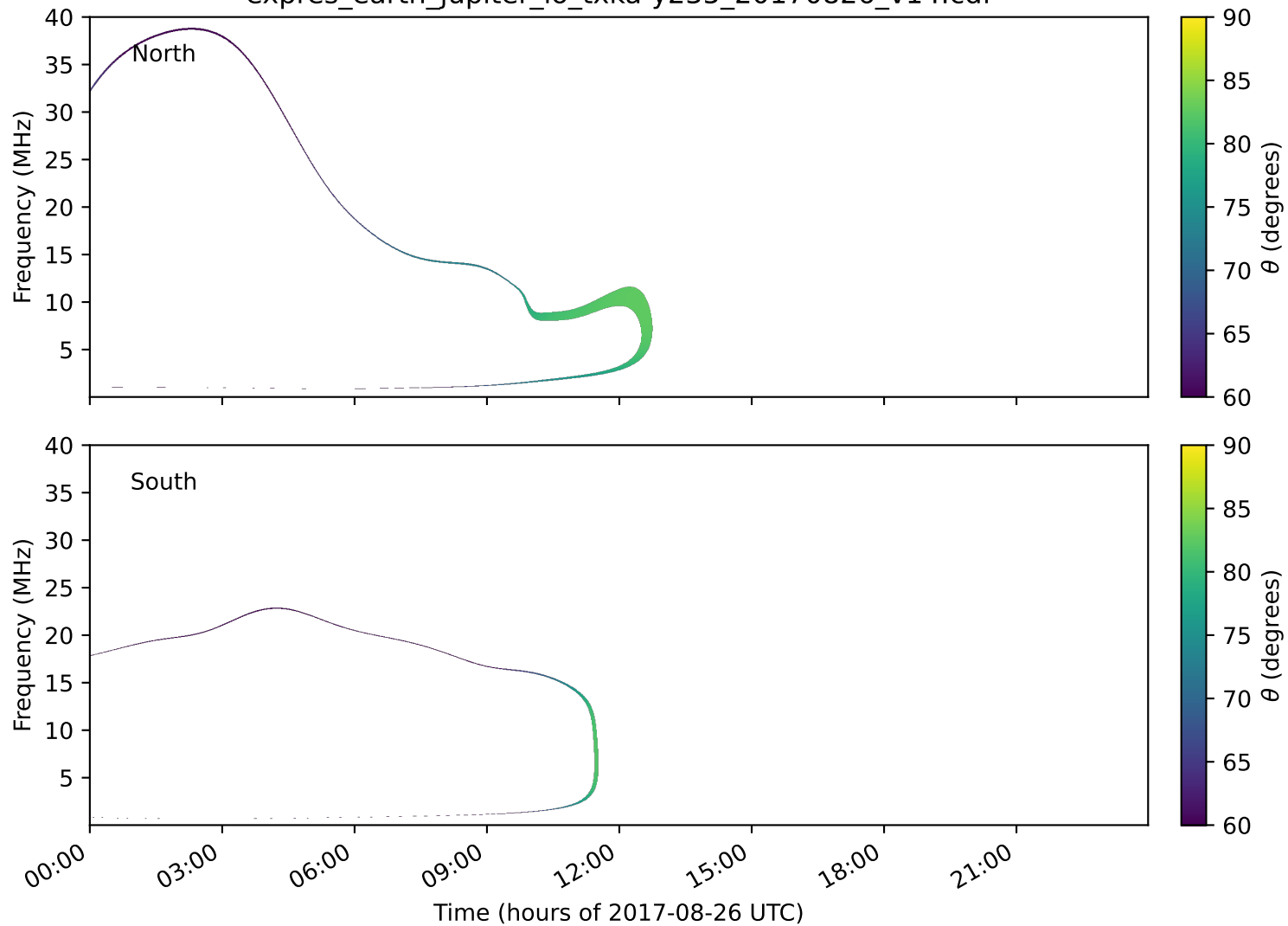
expres_earth_jupiter_io_txka-y235_20170826_v14.cdf
