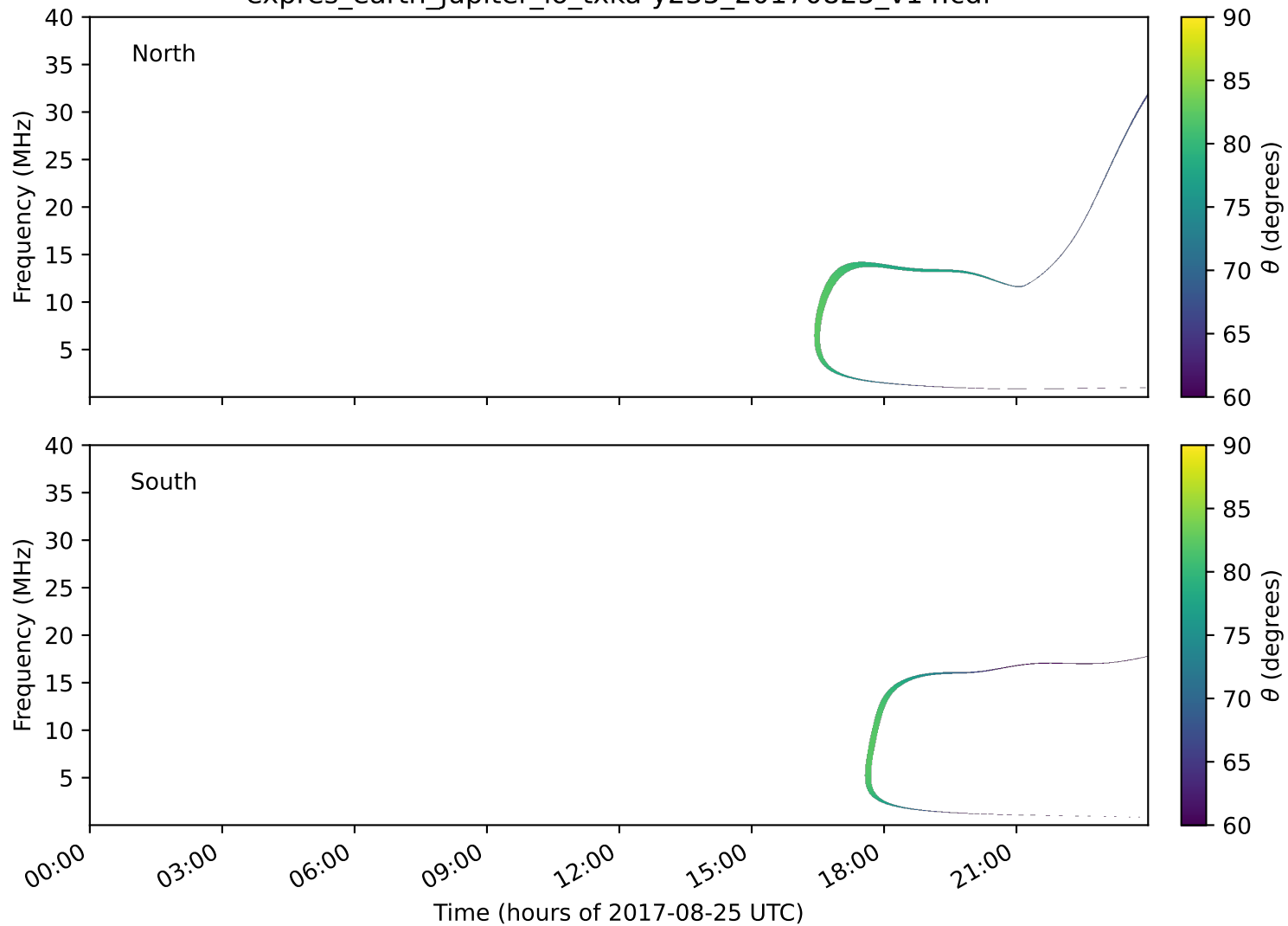
expres_earth_jupiter_io_txka-y235_20170825_v14.cdf
