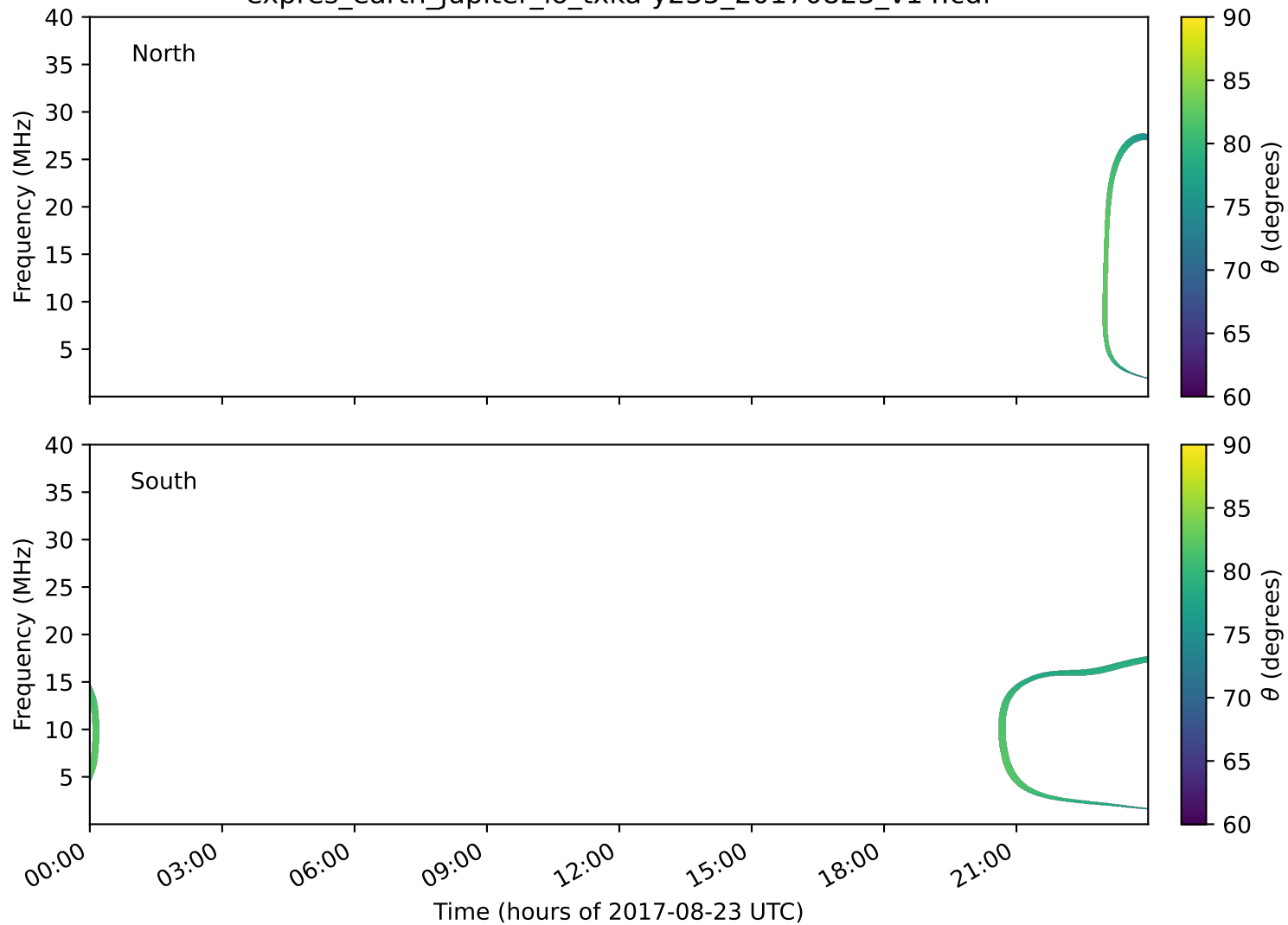
expres_earth_jupiter_io_txka-y235_20170823_v14.cdf
