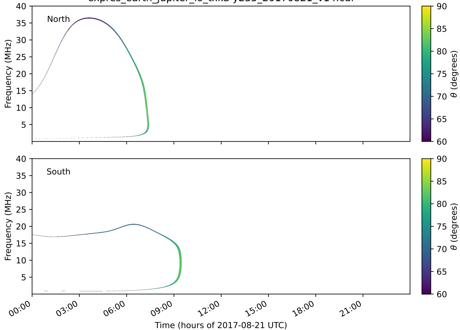
expres_earth_jupiter_io_txka-y235_20170821_v14.cdf
