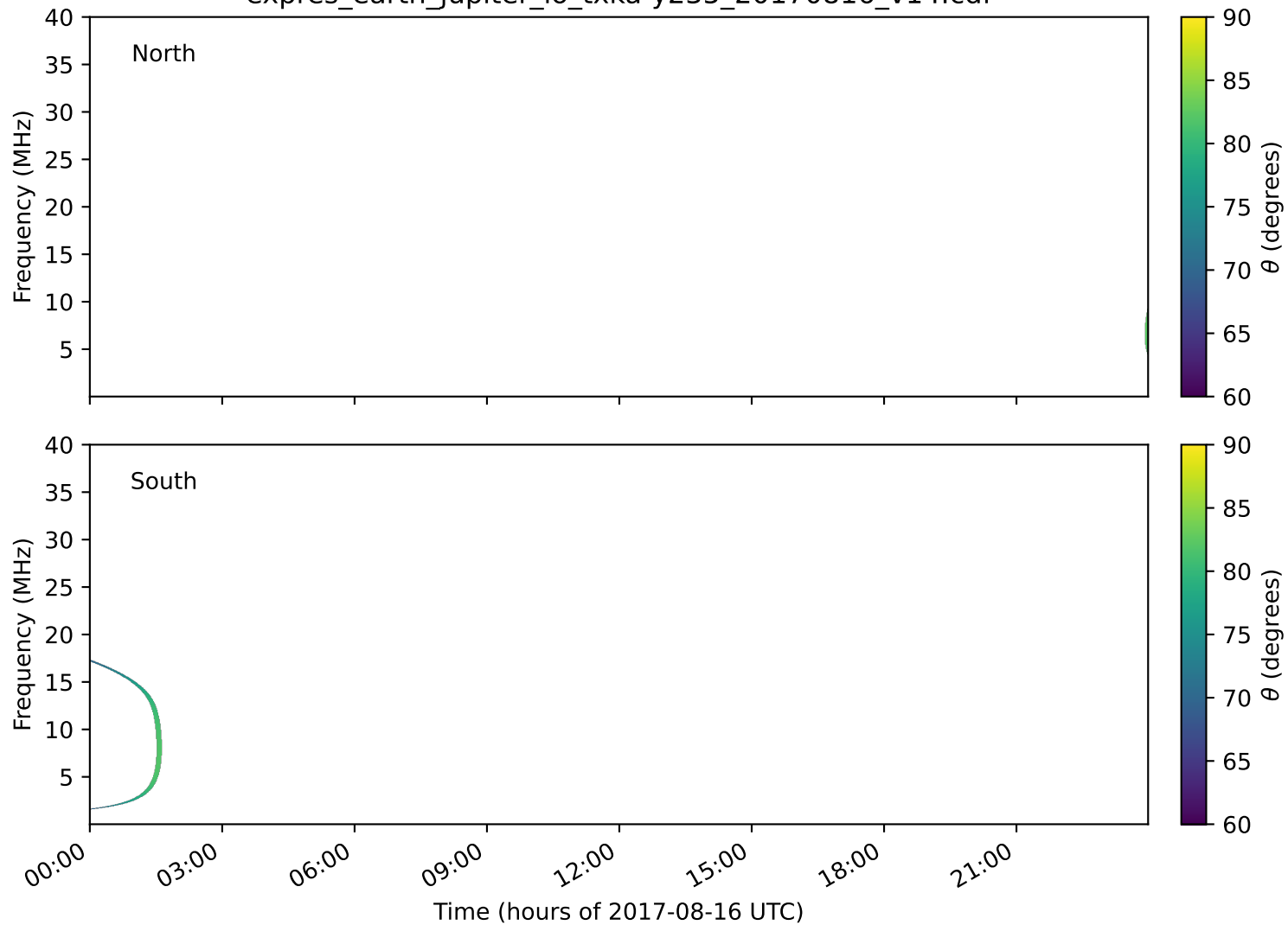
expres_earth_jupiter_io_txka-y235_20170816_v14.cdf
