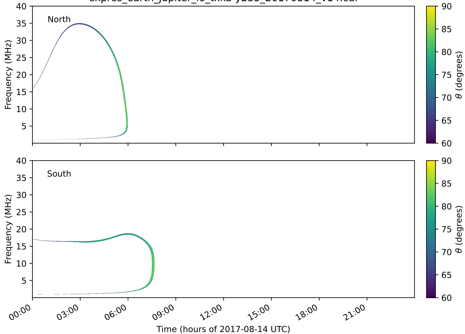
expres_earth_jupiter_io_txka-y235_20170814_v14.cdf
