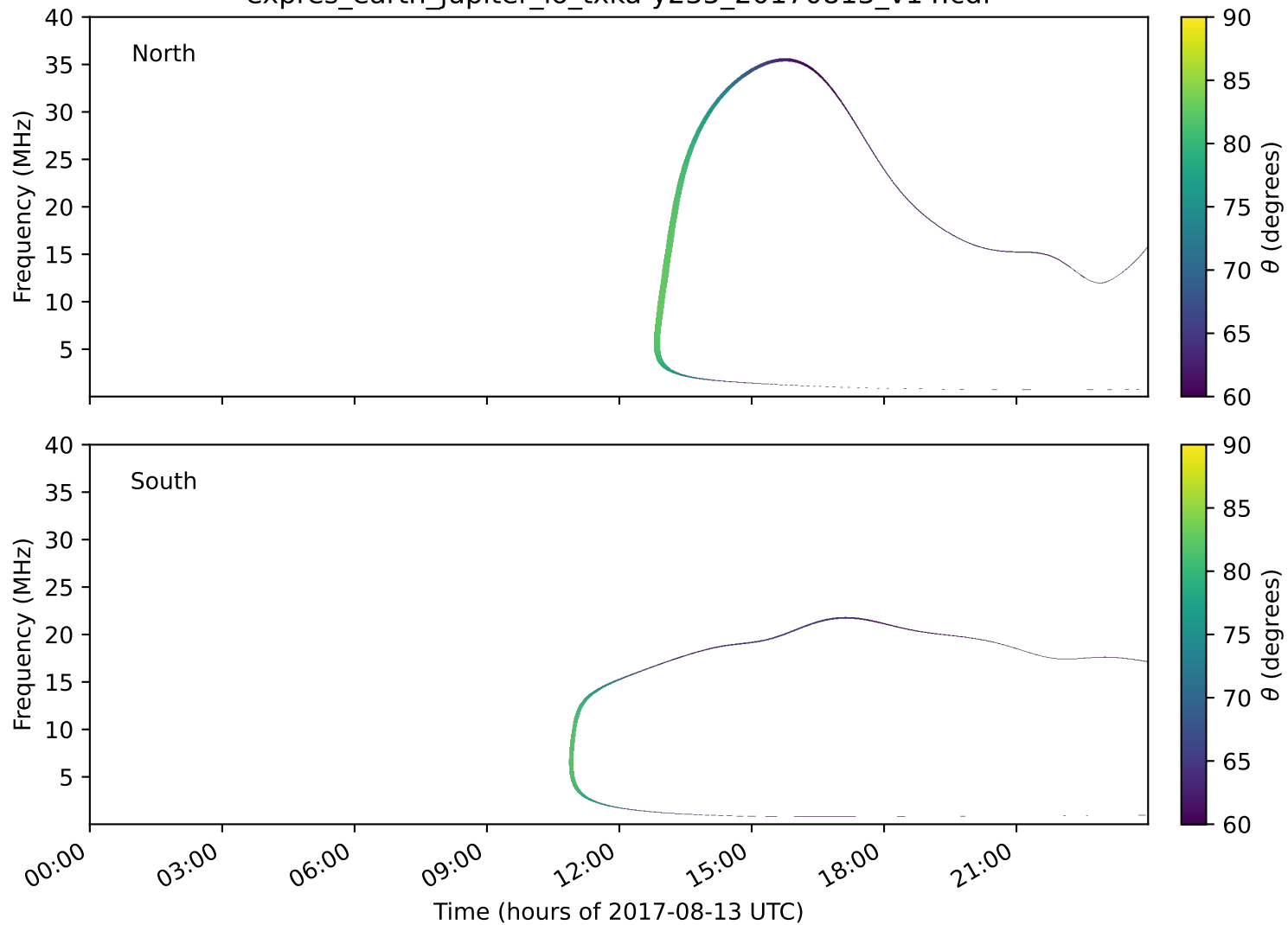
expres_earth_jupiter_io_txka-y235_20170813_v14.cdf
