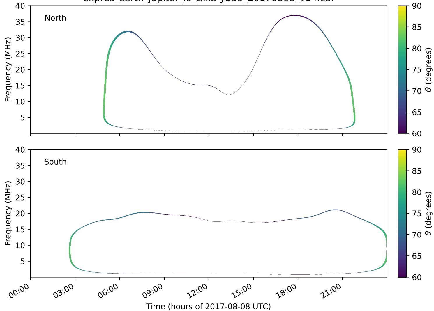
expres_earth_jupiter_io_txka-y235_20170808_v14.cdf
