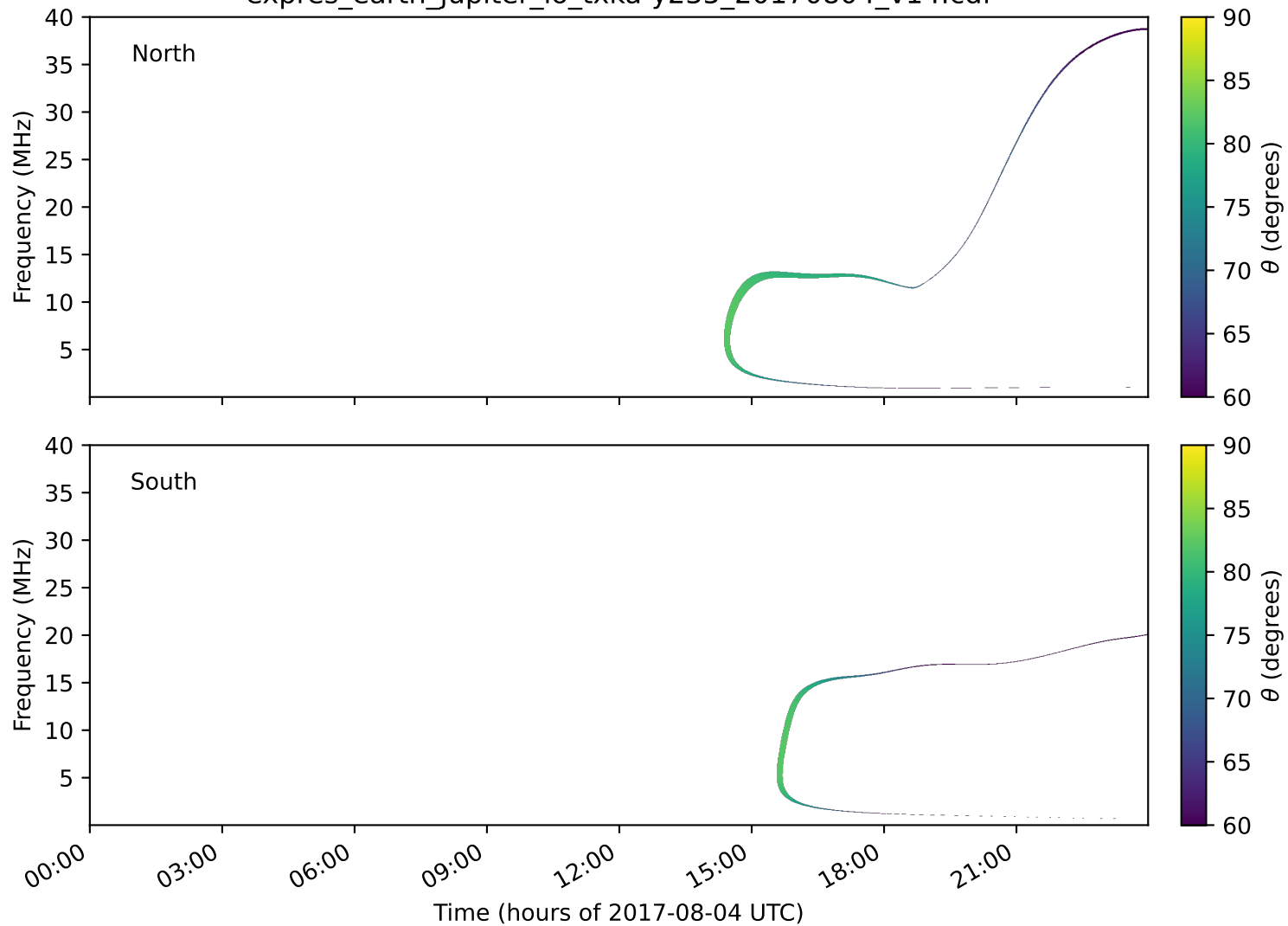
expres_earth_jupiter_io_txka-y235_20170804_v14.cdf
