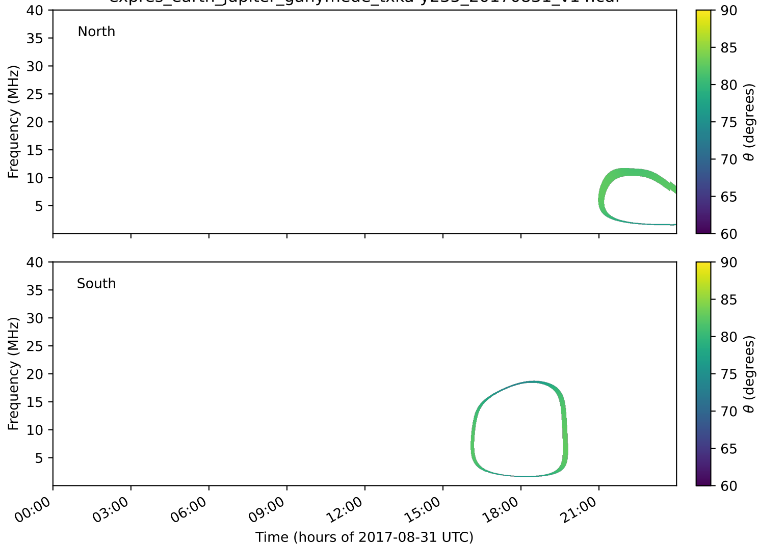
expres_earth_jupiter_ganymede_txka-y235_20170831_v14.cdf
