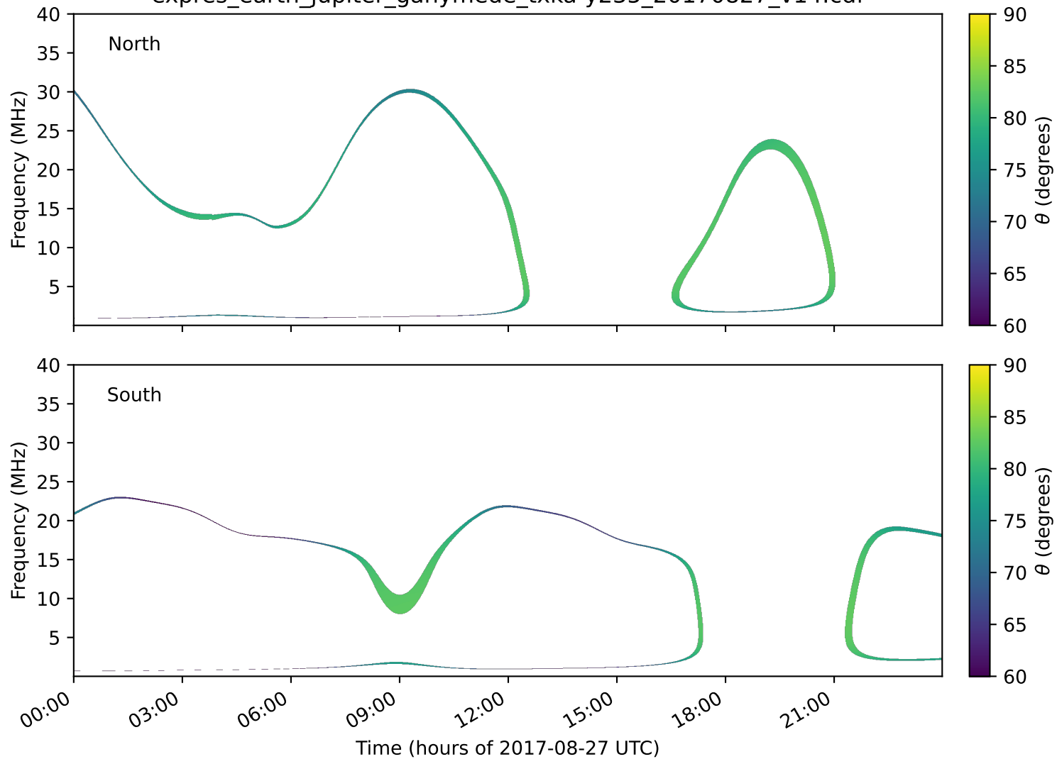
expres_earth_jupiter_ganymede_txka-y235_20170827_v14.cdf
