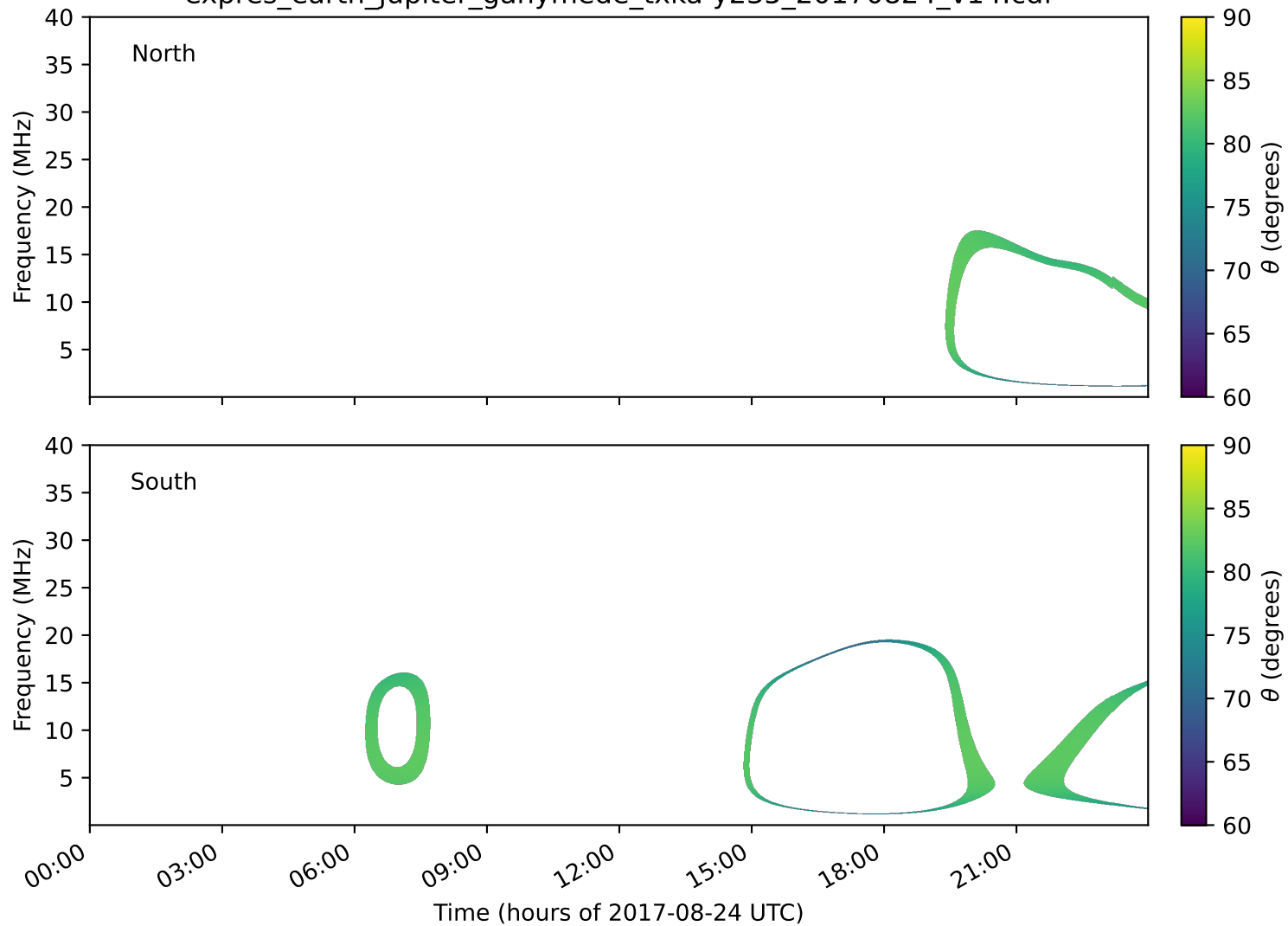
expres_earth_jupiter_ganymede_txka-y235_20170824_v14.cdf
