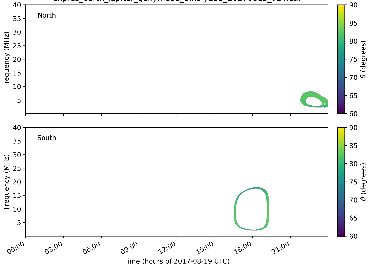
expres_earth_jupiter_ganymede_txka-y235_20170819_v14.cdf
