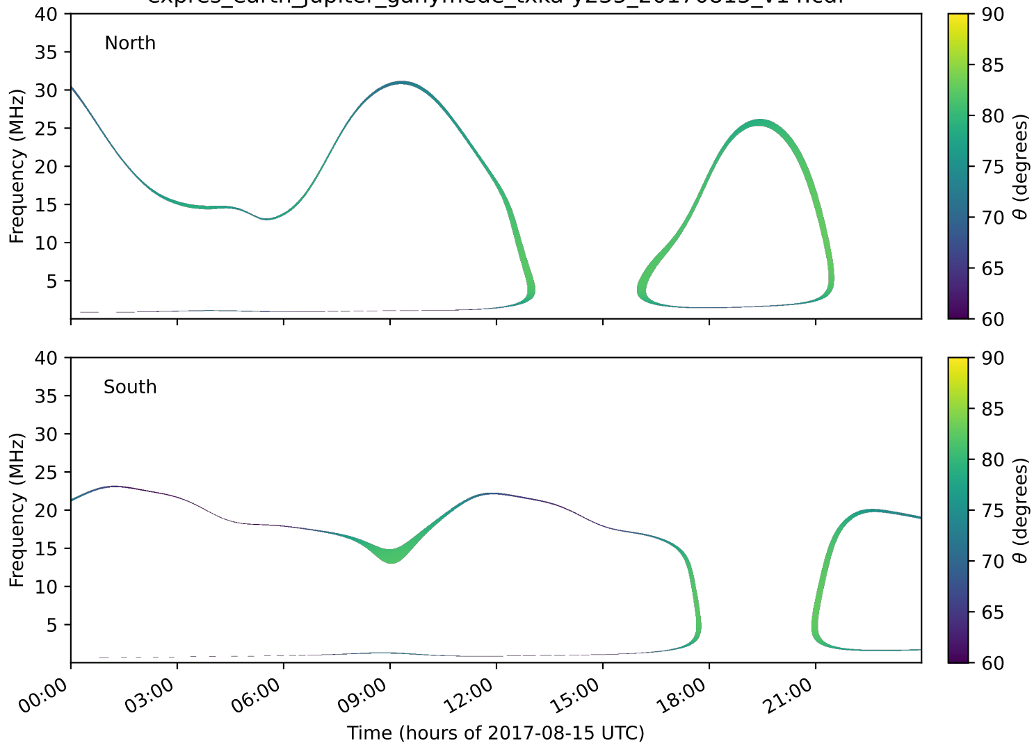
expres_earth_jupiter_ganymede_txka-y235_20170815_v14.cdf
