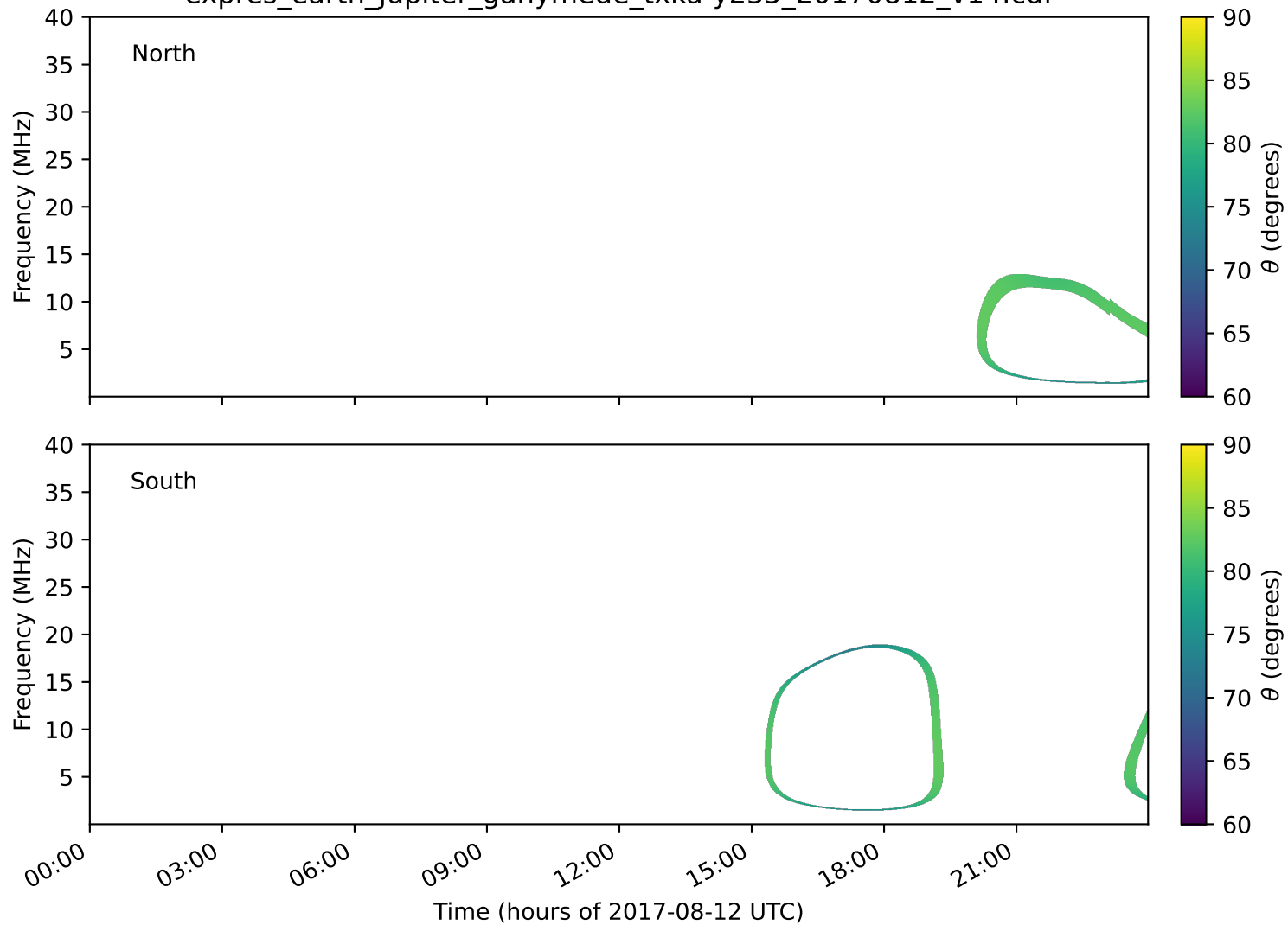
expres_earth_jupiter_ganymede_txka-y235_20170812_v14.cdf
