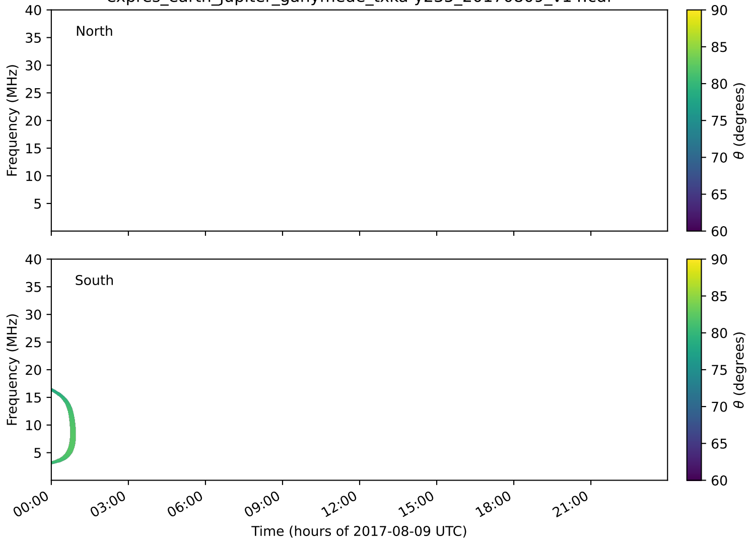
expres_earth_jupiter_ganymede_txka-y235_20170809_v14.cdf
