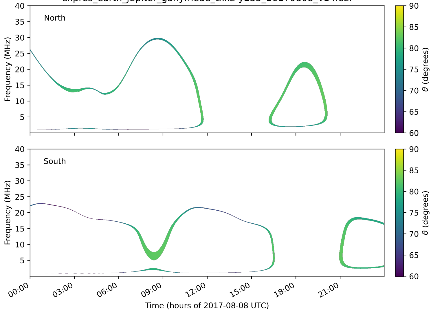
expres_earth_jupiter_ganymede_txka-y235_20170808_v14.cdf
