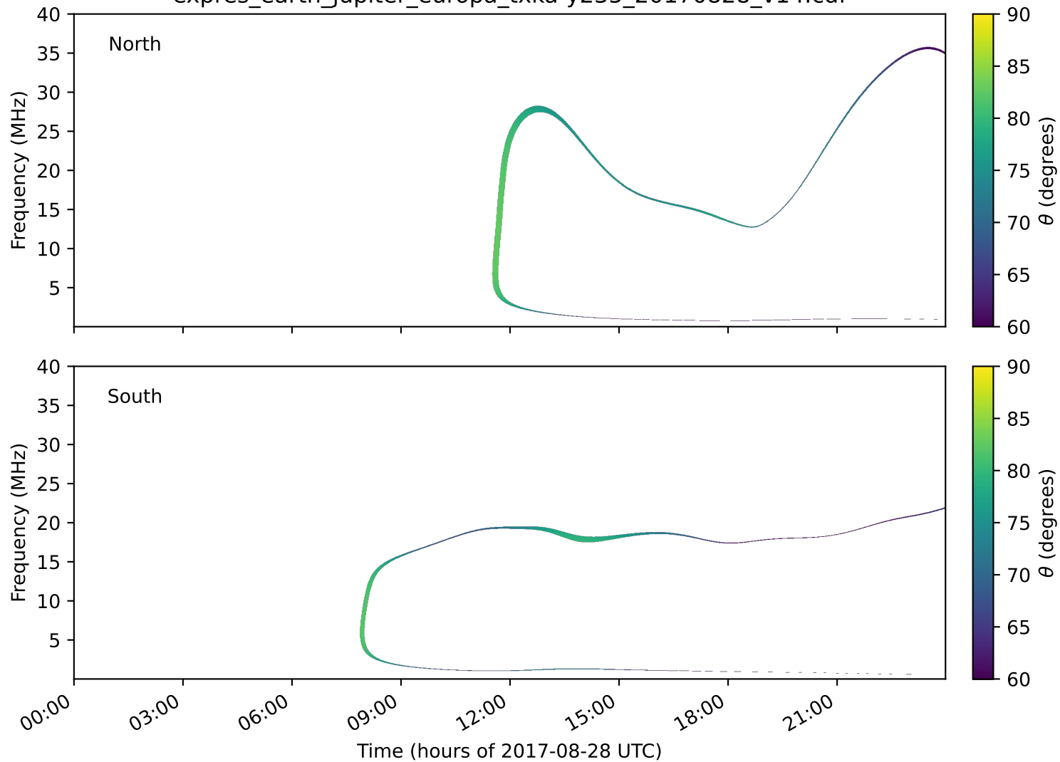
expres_earth_jupiter_europa_txka-y235_20170828_v14.cdf
