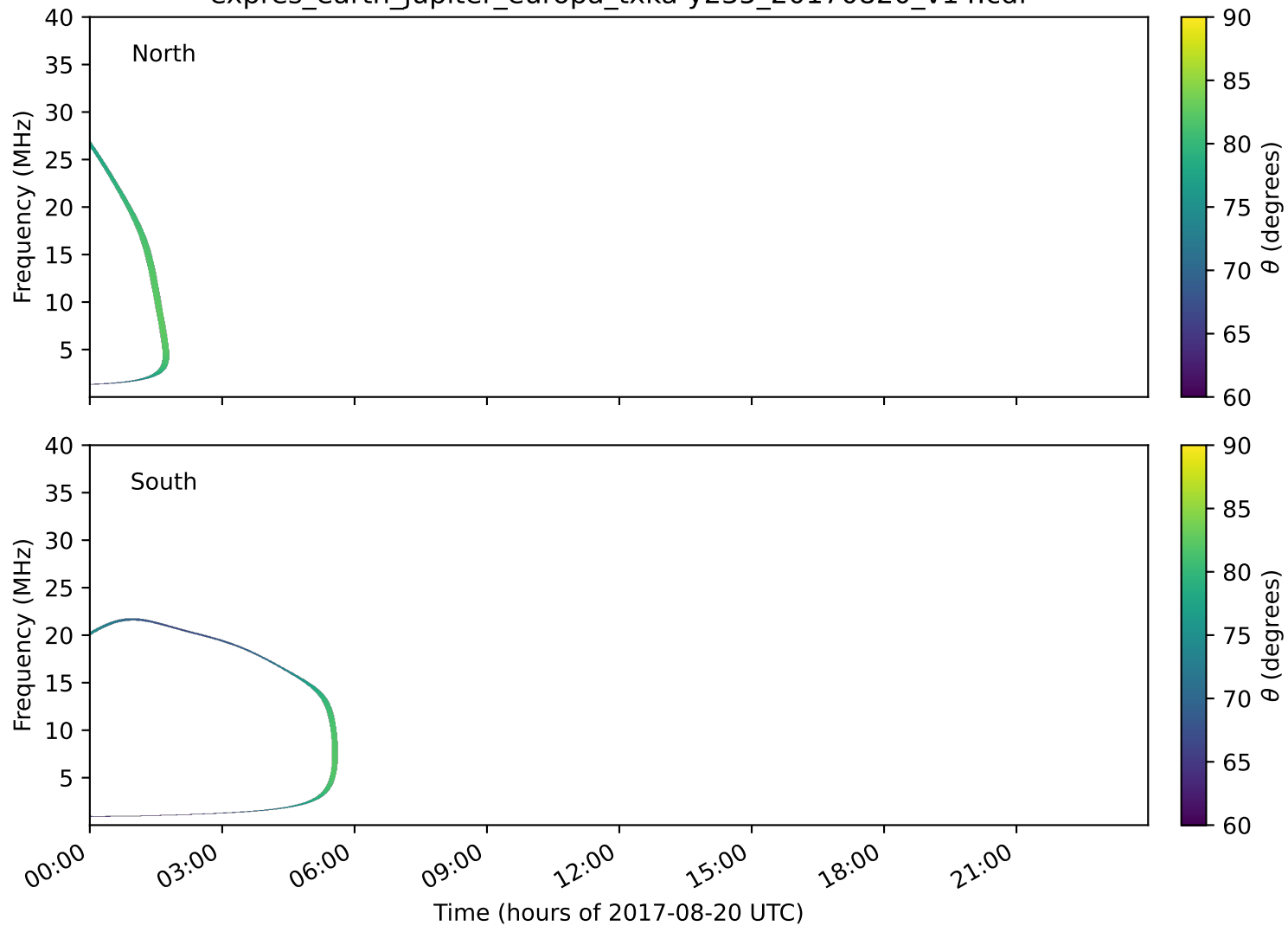
expres_earth_jupiter_europa_txka-y235_20170820_v14.cdf
