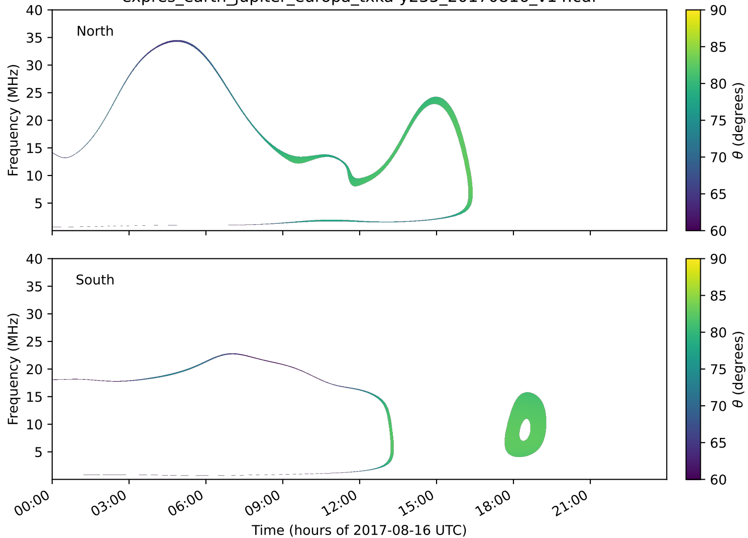
expres_earth_jupiter_europa_txka-y235_20170816_v14.cdf
