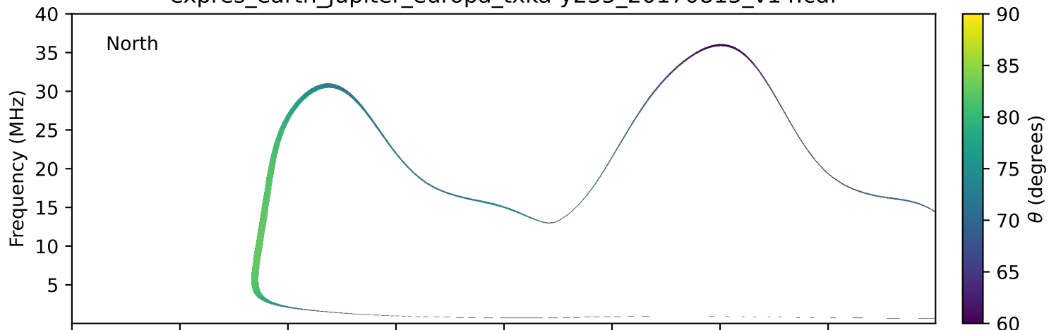
expres_earth_jupiter_europa_txka-y235_20170815_v14.cdf
