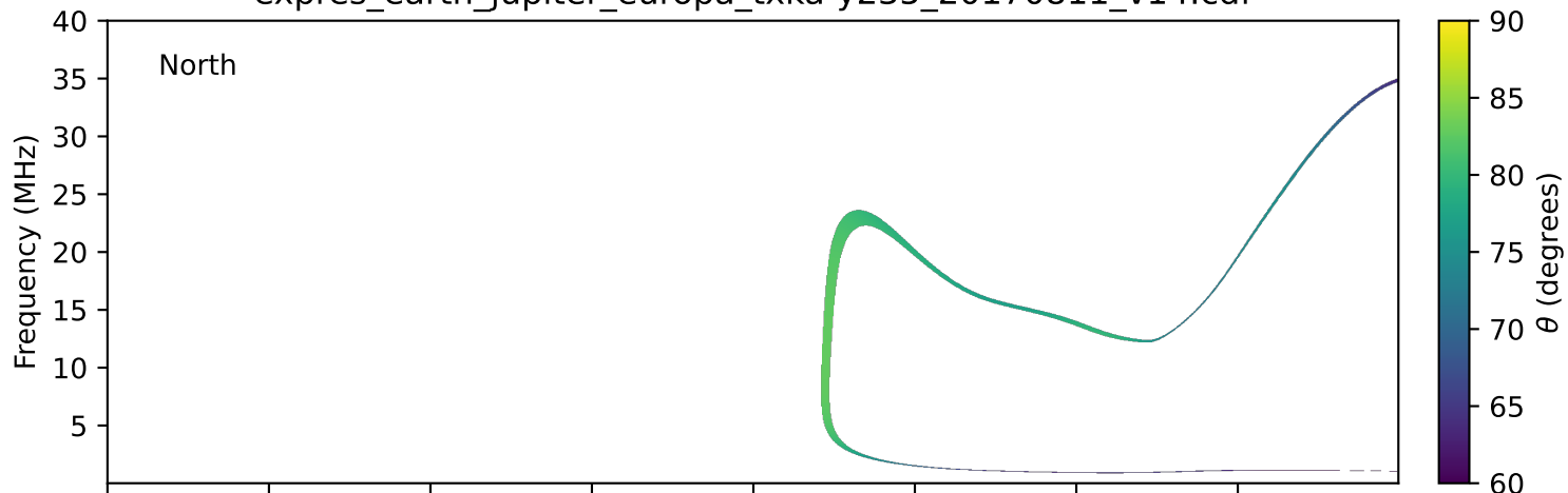
expres_earth_jupiter_europa_txka-y235_20170811_v14.cdf
