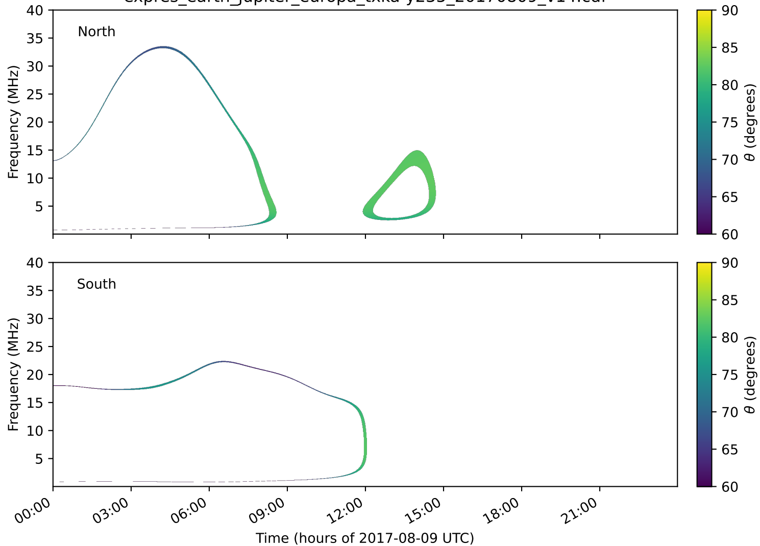
expres_earth_jupiter_europa_txka-y235_20170809_v14.cdf
