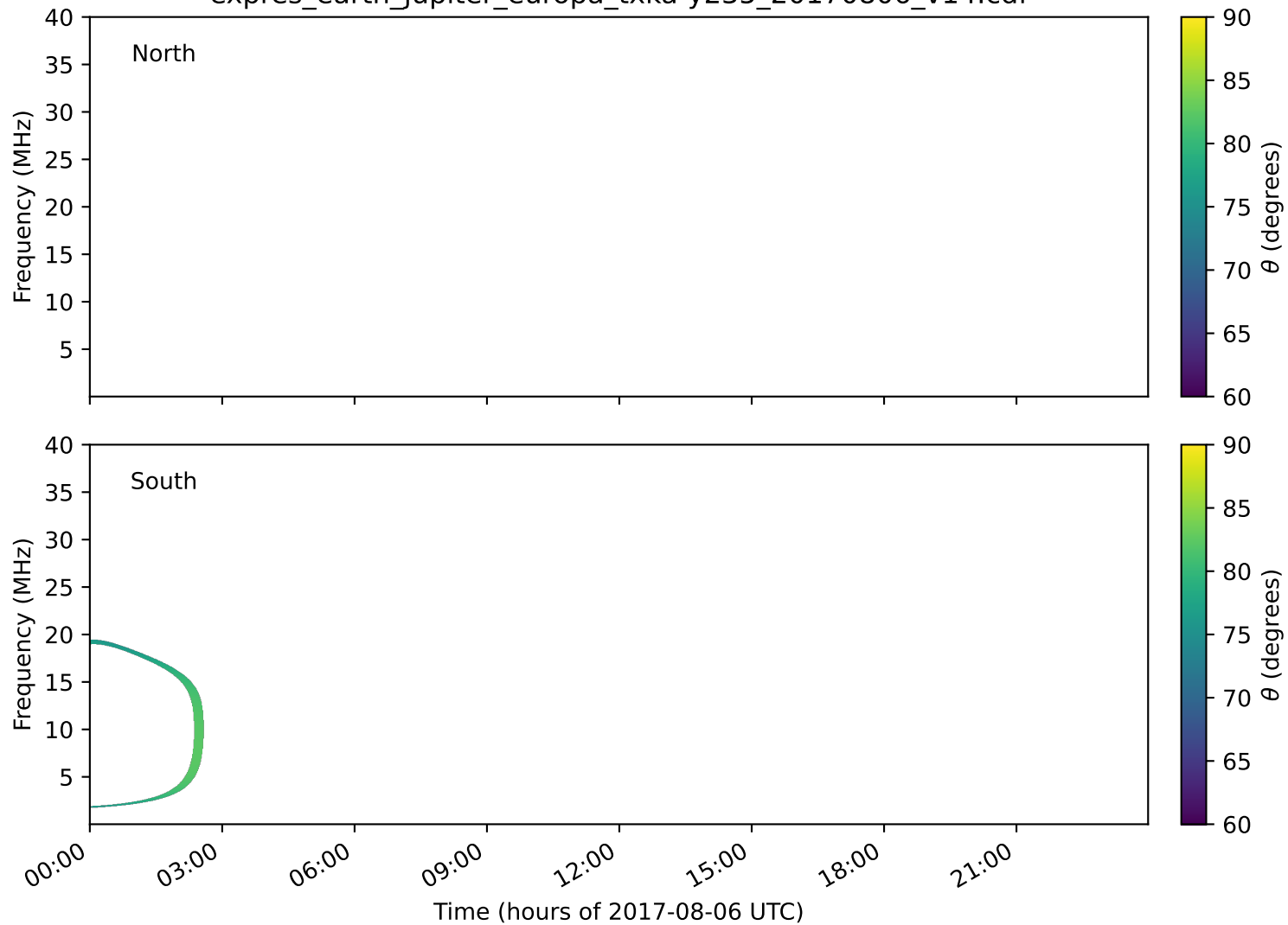
expres_earth_jupiter_europa_txka-y235_20170806_v14.cdf
