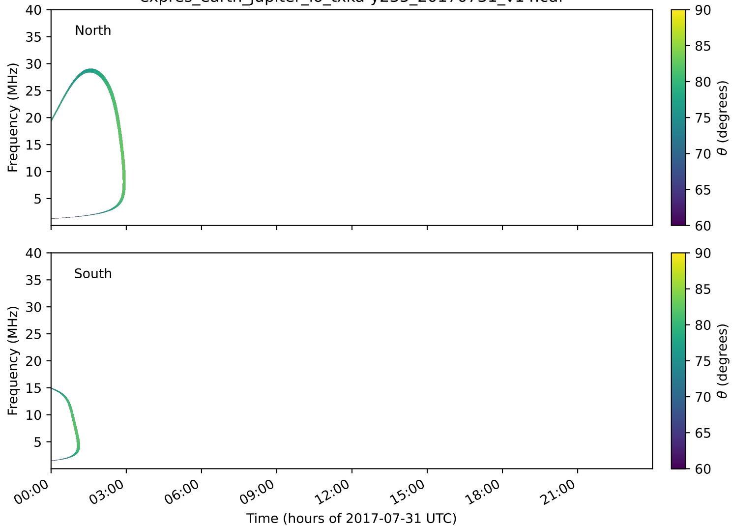
expres_earth_jupiter_io_txka-y235_20170731_v14.cdf
