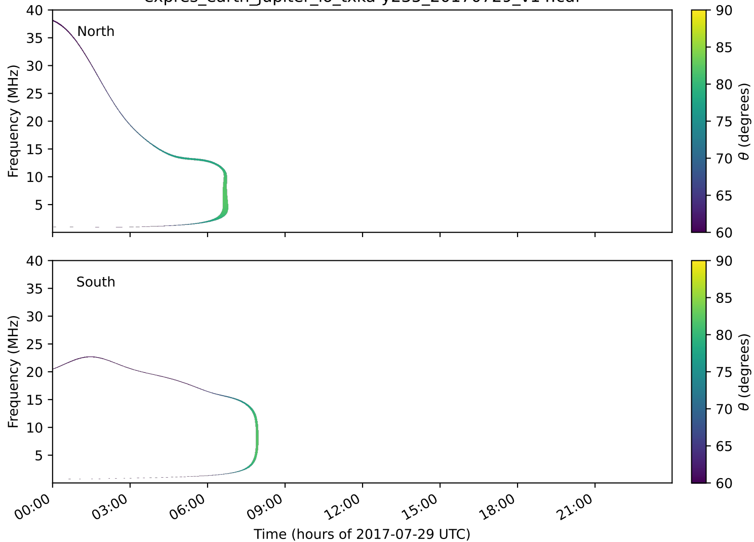
expres_earth_jupiter_io_txka-y235_20170729_v14.cdf
