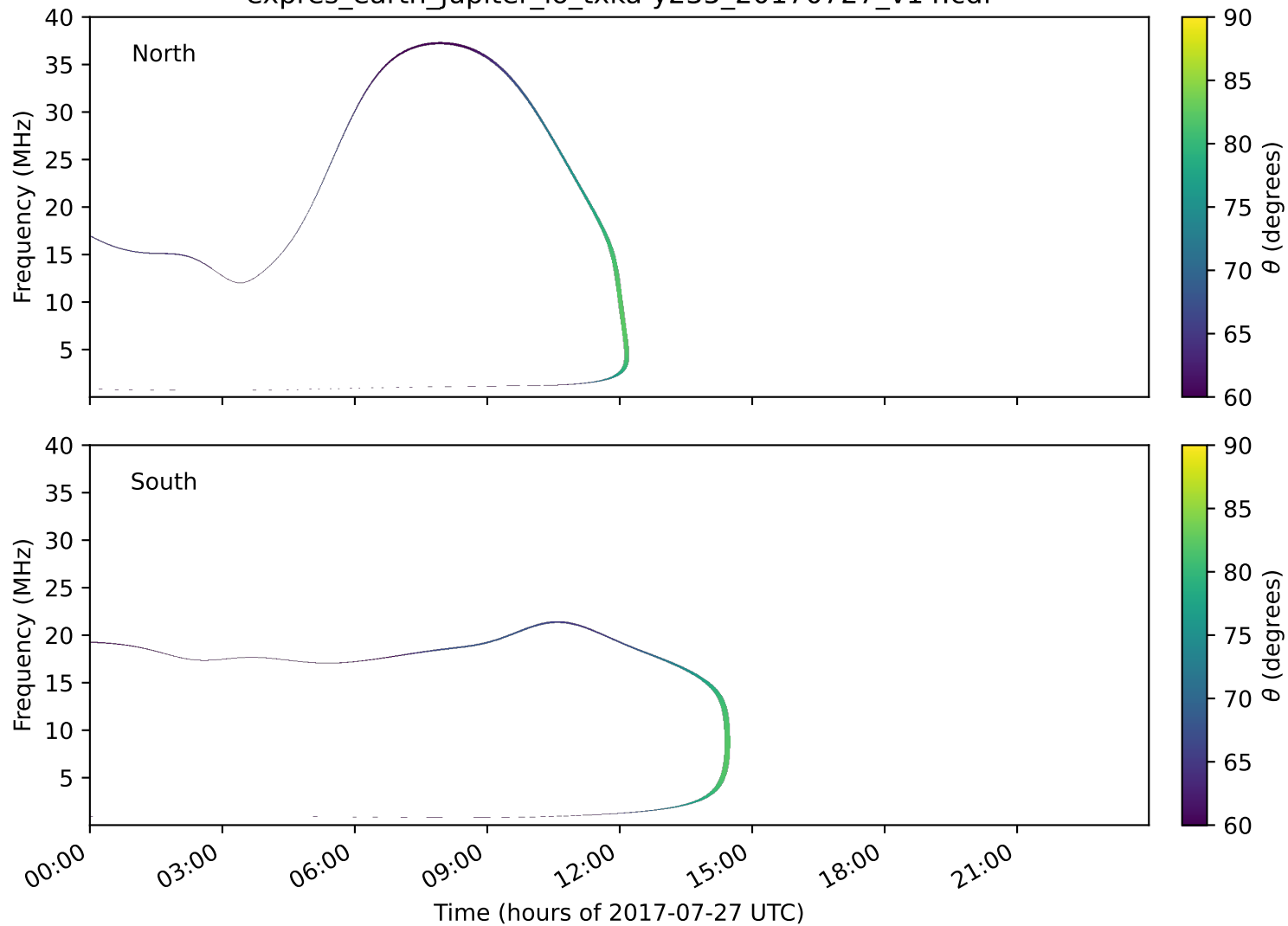
expres_earth_jupiter_io_txka-y235_20170727_v14.cdf
