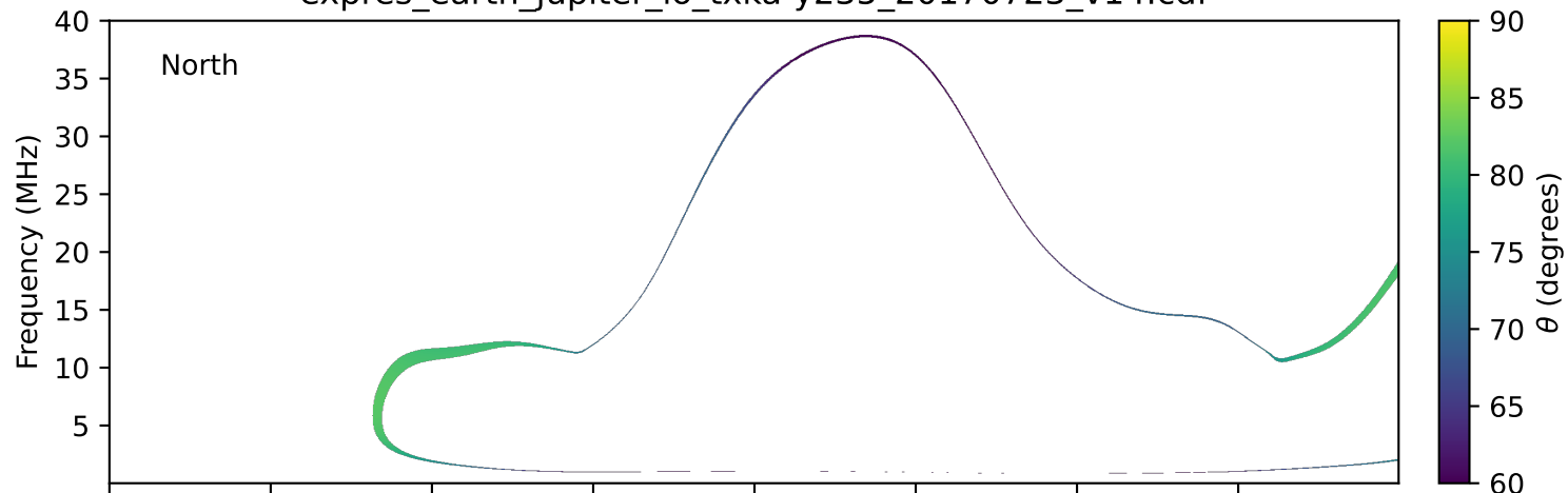
expres_earth_jupiter_io_txka-y235_20170723_v14.cdf
