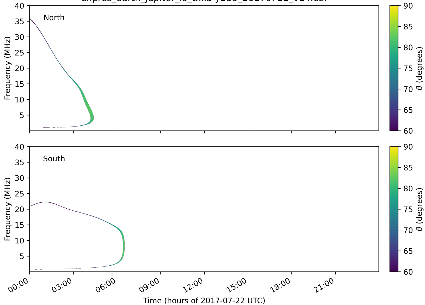
expres_earth_jupiter_io_txka-y235_20170722_v14.cdf
