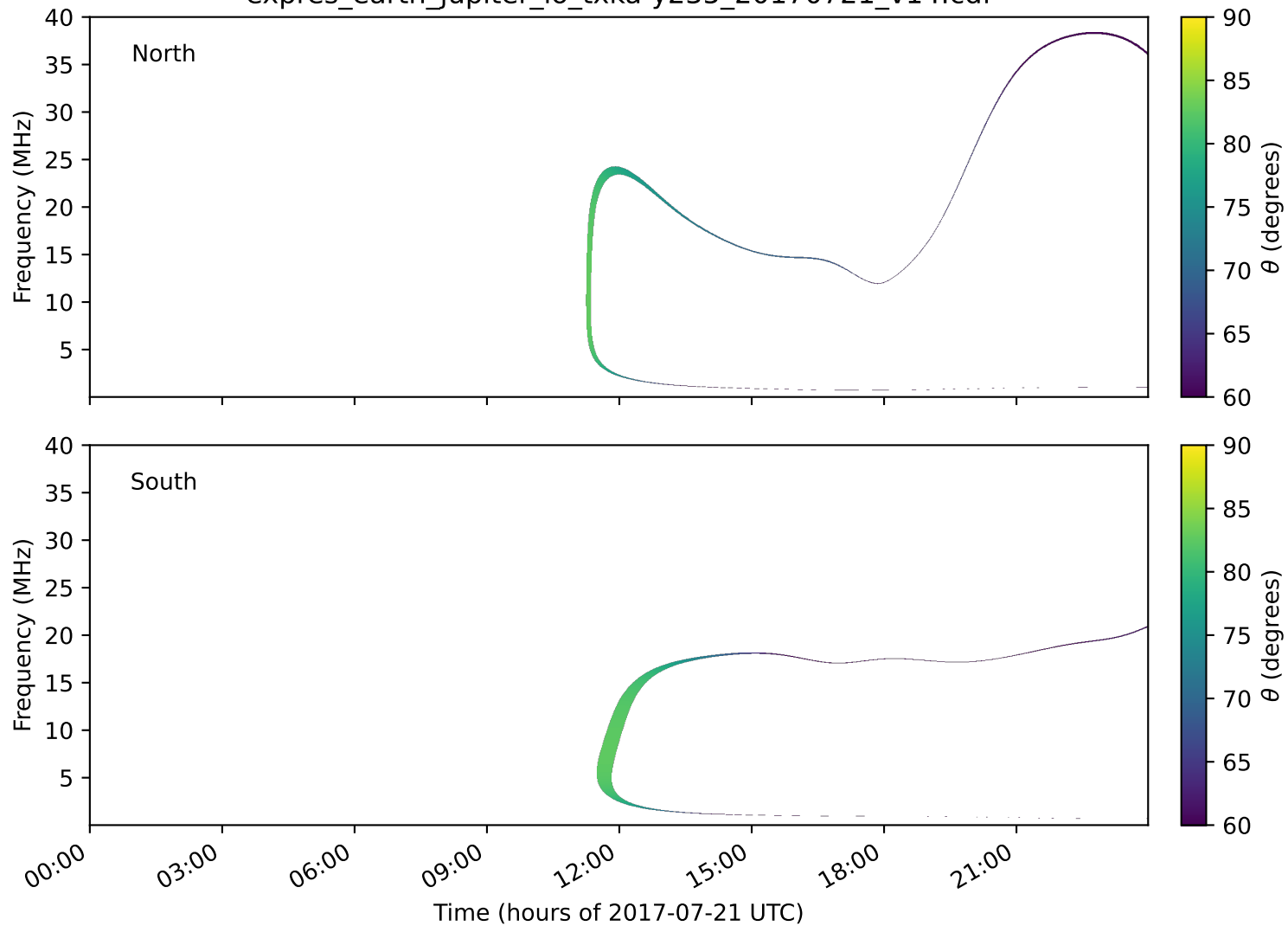
expres_earth_jupiter_io_txka-y235_20170721_v14.cdf
