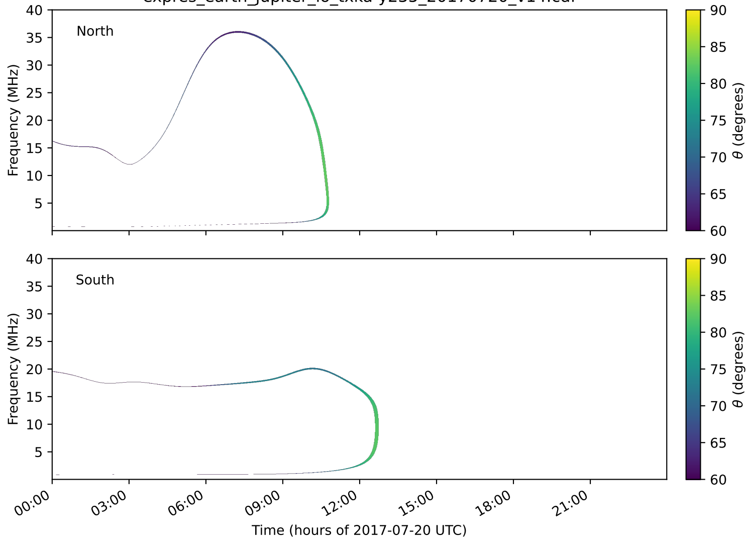
expres_earth_jupiter_io_txka-y235_20170720_v14.cdf
