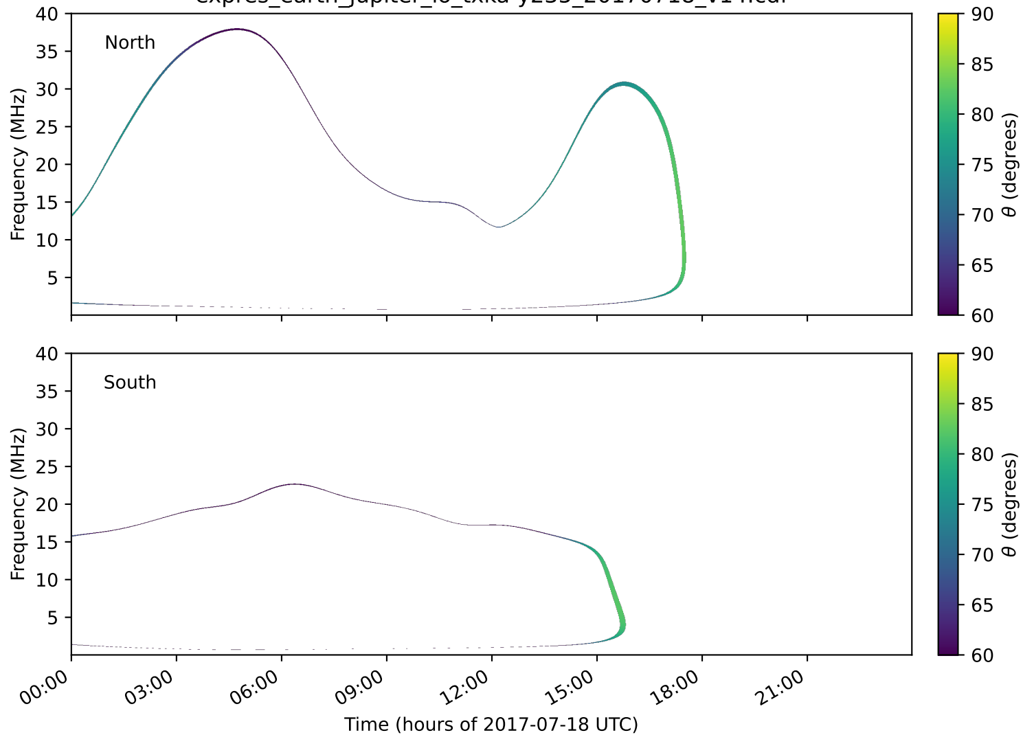
expres_earth_jupiter_io_txka-y235_20170718_v14.cdf
