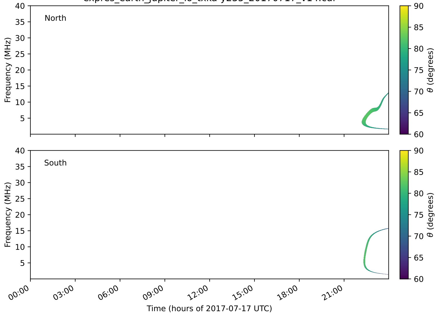
expres_earth_jupiter_io_txka-y235_20170717_v14.cdf
